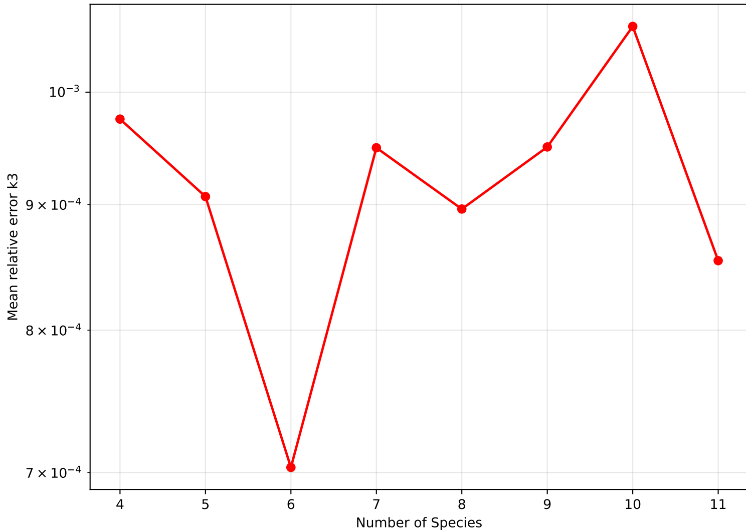
50, 50 — Mean relative error k3 vs number of species (zoomed: 4 to 11 species)
